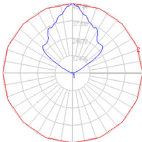
Test: ETL Photometric 684 Watt including ballasts.
